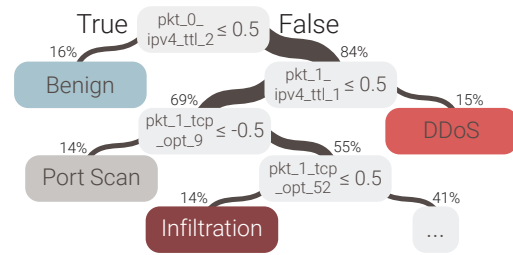
Figure 6: Decision tree for nPrintML IDS model.
