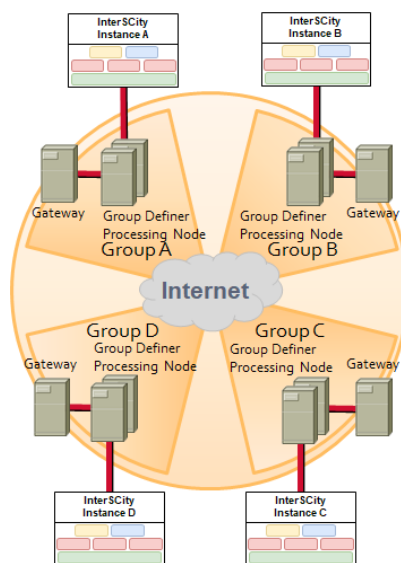
Figure 5: MUSANet: Multi-domain InterSCity-ContextNet pairs
