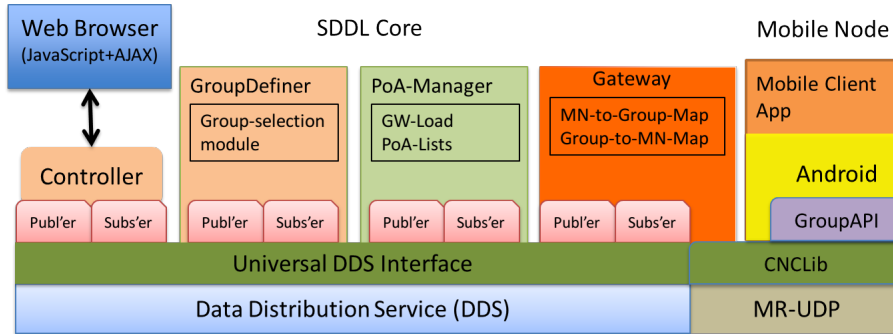
Figure 1: SDDL Components Pre-IoMT
