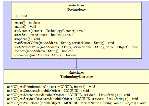
Figure 2: Main two interfaces of the S2PA
